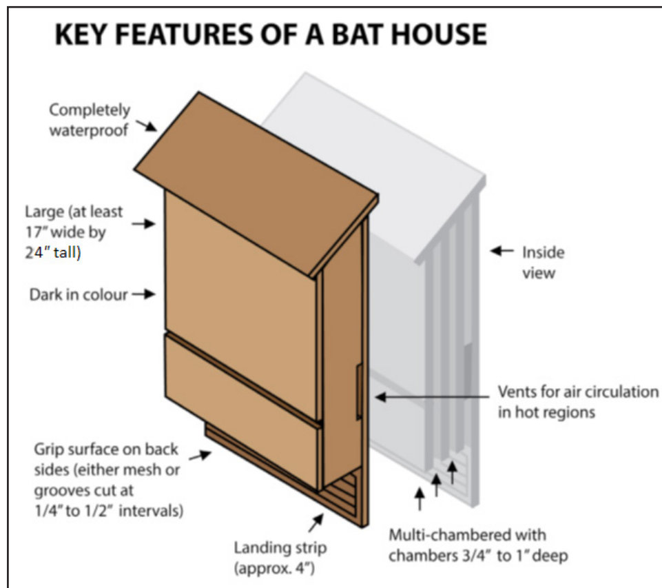
Figure 62. General guidelines for multi-chambered bat boxes.
